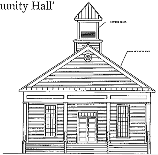
CHAPEL FRONT ELEVATION SCALE: 3/16"=1'-0"
