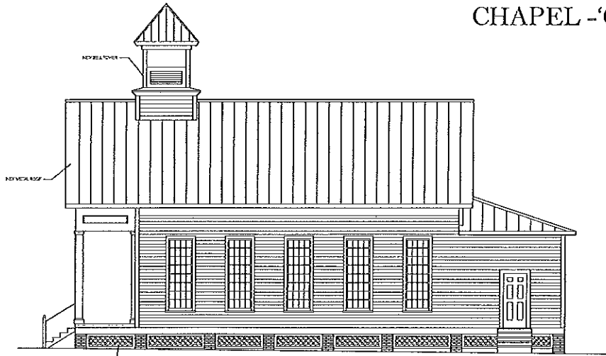
CHAPEL SIDE ELEVATION SCALE: 3/16"=1'-0"
